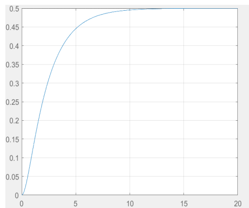
Gambar 3. 6 Kurva Overdamped
