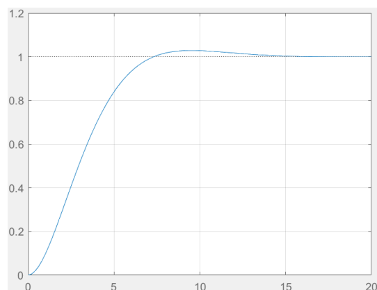
Gambar 3. 4 Kurva Underdamped
