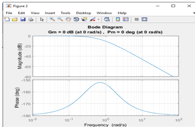
Gambar 4. 14 Diagram Bode Keadaan Stabil Marginal
