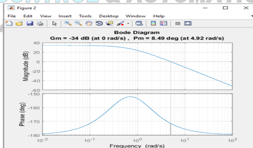
Gambar 4. 15 Diagram Bode Keadaan Stabil Marginal
