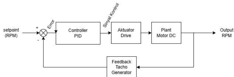
Gambar 5. 3 Diagram Blok PID
