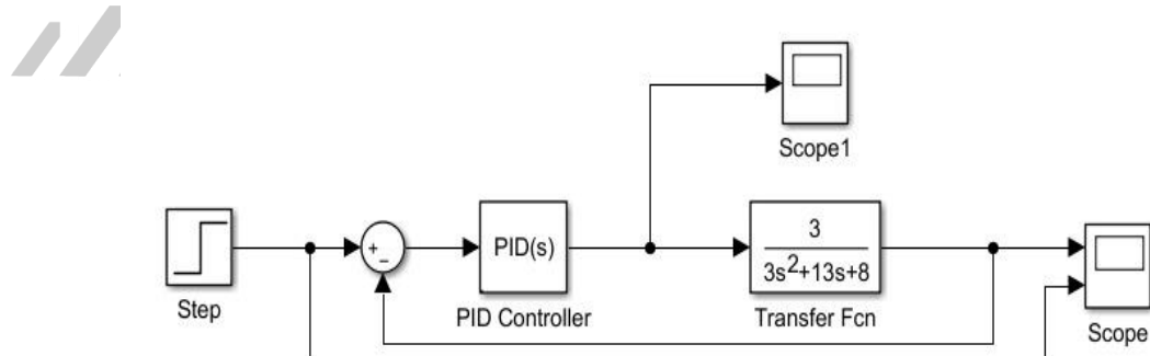
Gambar 5. 4 Diagram Blok Close Loop PID
