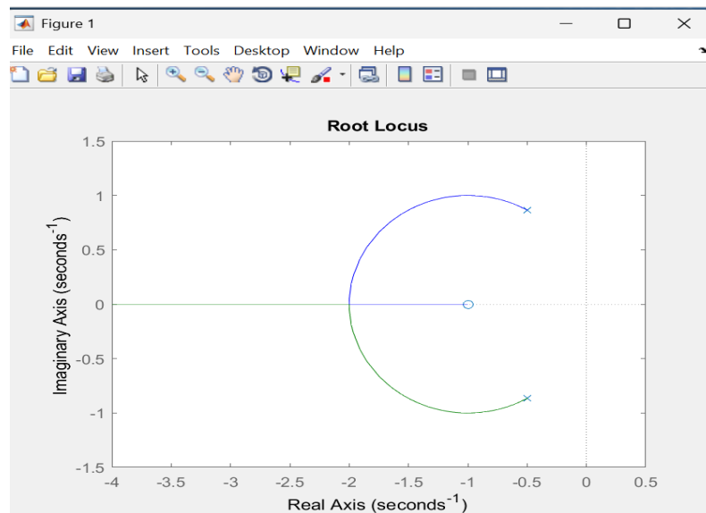
Gambar 4. 7 Keadaan Stabil
