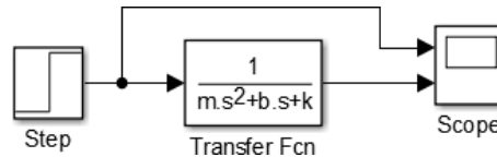
Gambar 3. 22 Diagram Blok
