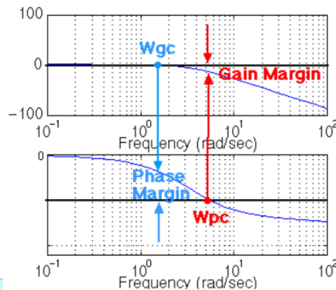
Gambar 4. 12 Bode Diagram
