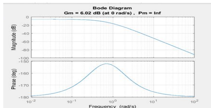
Gambar 4. 13 Bode Plot Keadaan Stabil
