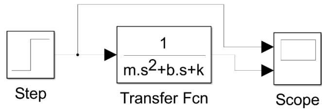
Gambar 3. 19 Diagram Blok
