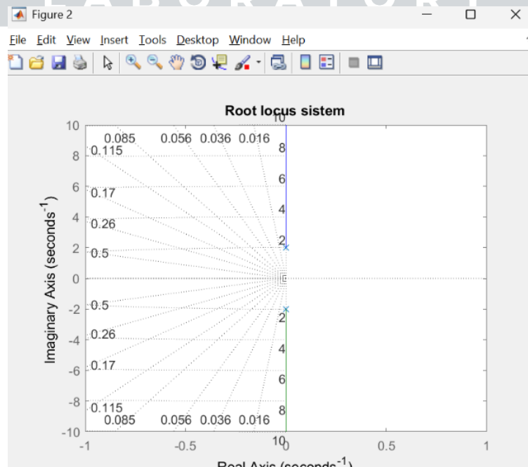
Gambar 4. 8 Keadaan Stabil Marginal
